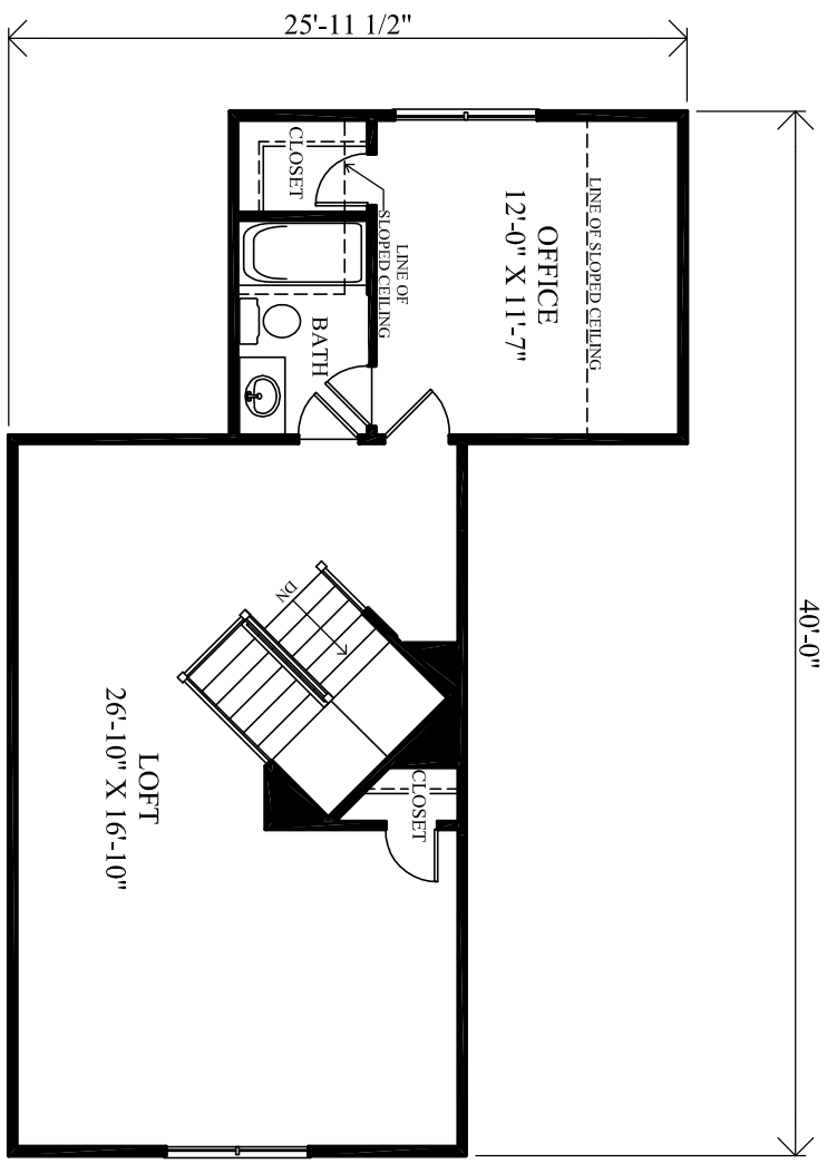
OPT. LOFT FLOOR PLAN
