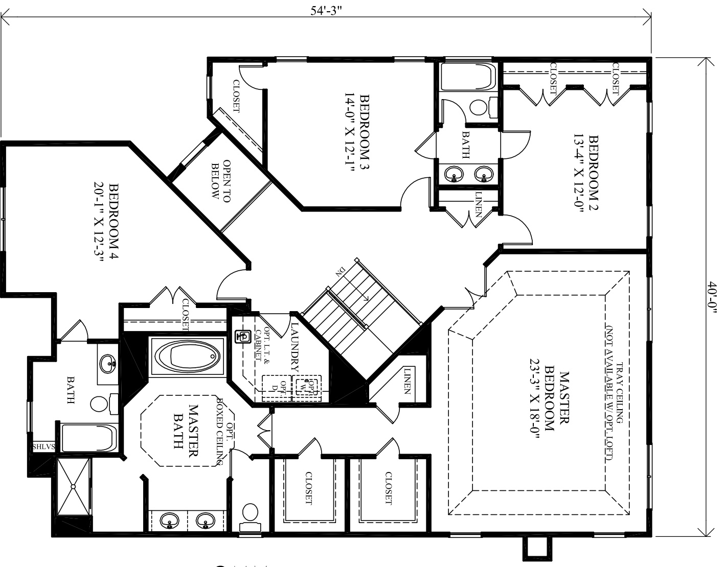
PARTIAL SECOND FLOOR PLAN W/ OPT. LOFT FLOOR PLAN
